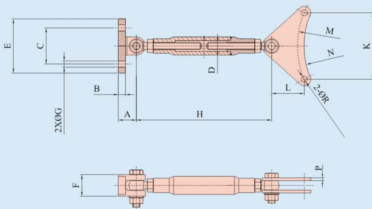
Accessory Dimensions
